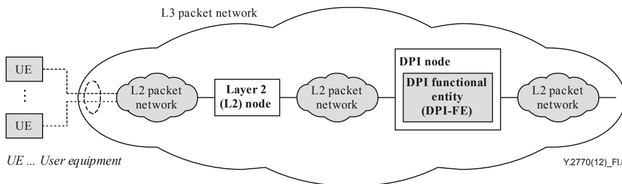
Figure I.8 – Network- vs Link-oriented DPI
