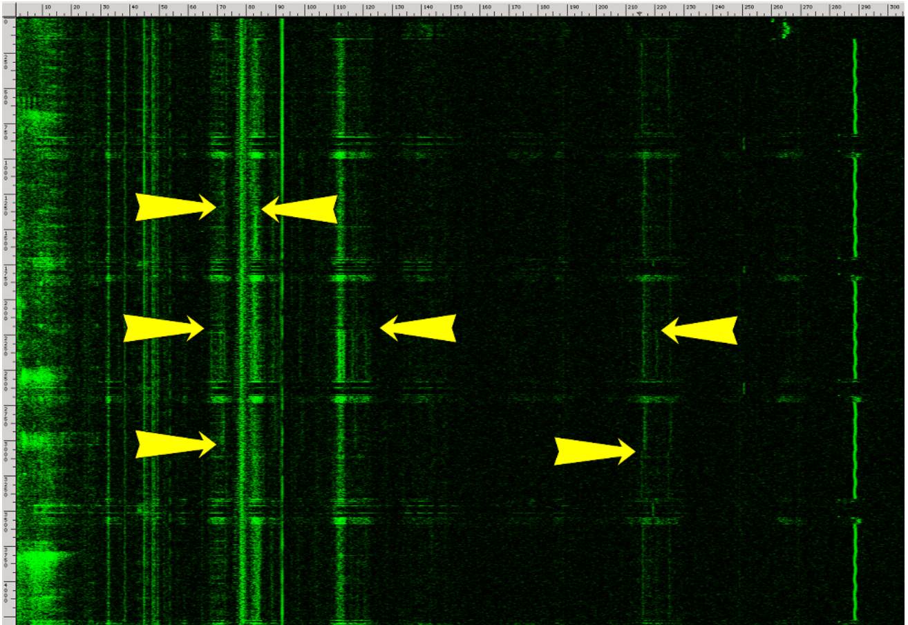
Figure 14: Acoustic signature (4 sec, 0–300 kHz) of five GnuPG RSA signatures executed on Evo N200. The recording was made using the lab-grade setup and the Brüel&Kjær 4939 high-frequency microphone capsule. The transitions between p and q are marked with yellow arrows.
