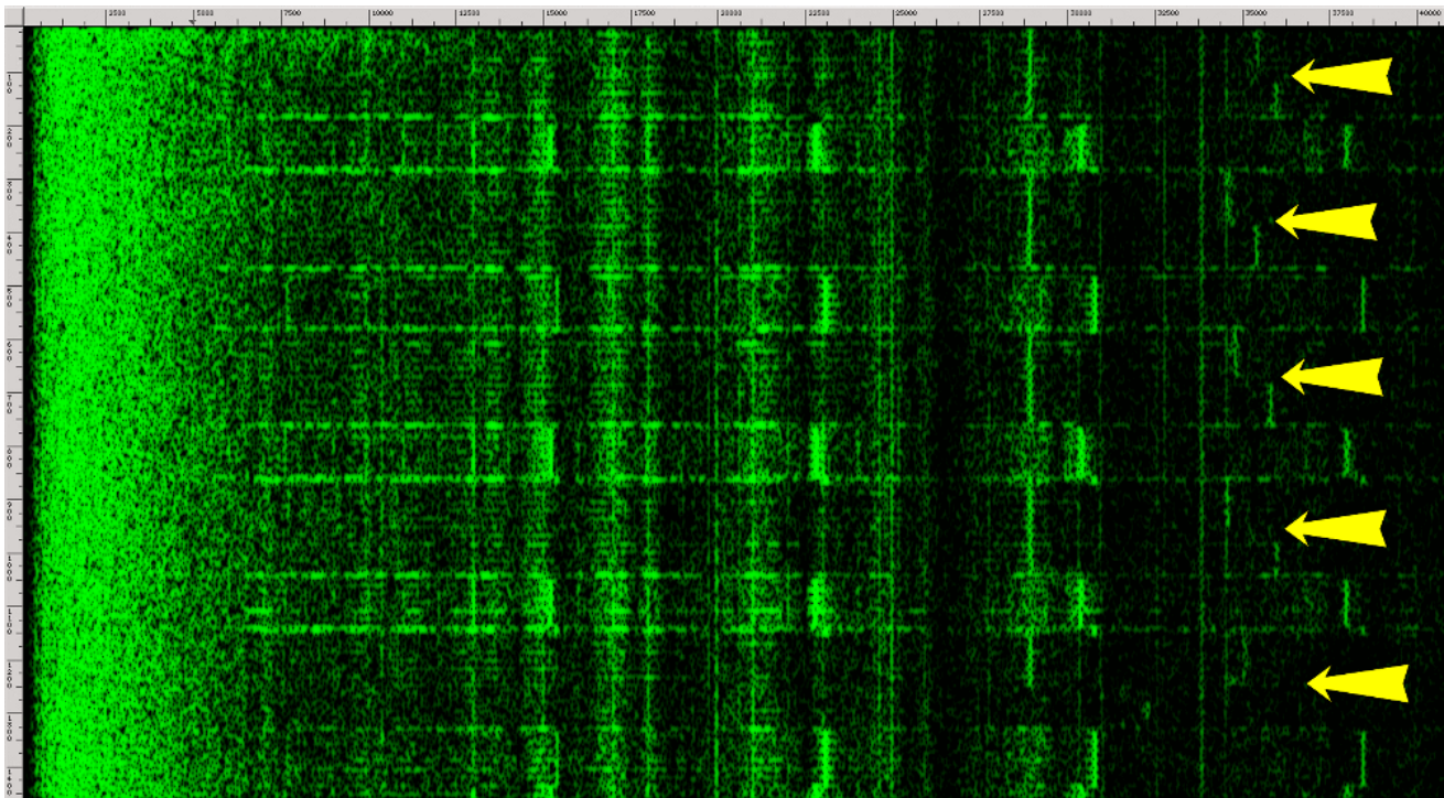
Figure 15: Acoustic signature (1.4 sec, 0–40 kHz) of five GnuPG RSA signatures executed on a Lenovo ThinkPad T61. The recording was made using the lab-grade setup and the Brüel&Kjær 4190 microphone capsule. The transitions between p and q are marked with yellow arrows.
