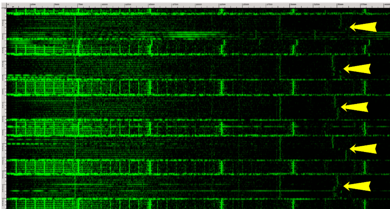
Figure 31: Power measurement FFT spectrogram of a recording (1.4 sec, 0–40 kHz) of five GnuPG RSA signatures executed on a Lenovo ThinkPad T61 using power analysis. The transitions between p and q are marked with yellow arrows.
