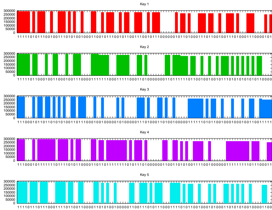
Figure 18: Number of zero limbs in the second operand of MUL\_BASECASE(a, b) during an execution of the modular exponentiation routine with the secret prime q using our attack and randomly generated keys. The correct bit values are indicated on the horizontal axis of each key.
