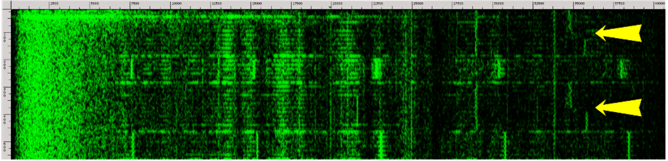
Figure 13: Acoustic signature (0.5 sec, 0–40 kHz) of two GnuPG RSA signatures executed on Lenovo ThinkPad T61. The recording was made using the lab-grade setup and the Brüel&Kjær 4190 microphone capsule. The transitions between p and q are marked with yellow arrows.
