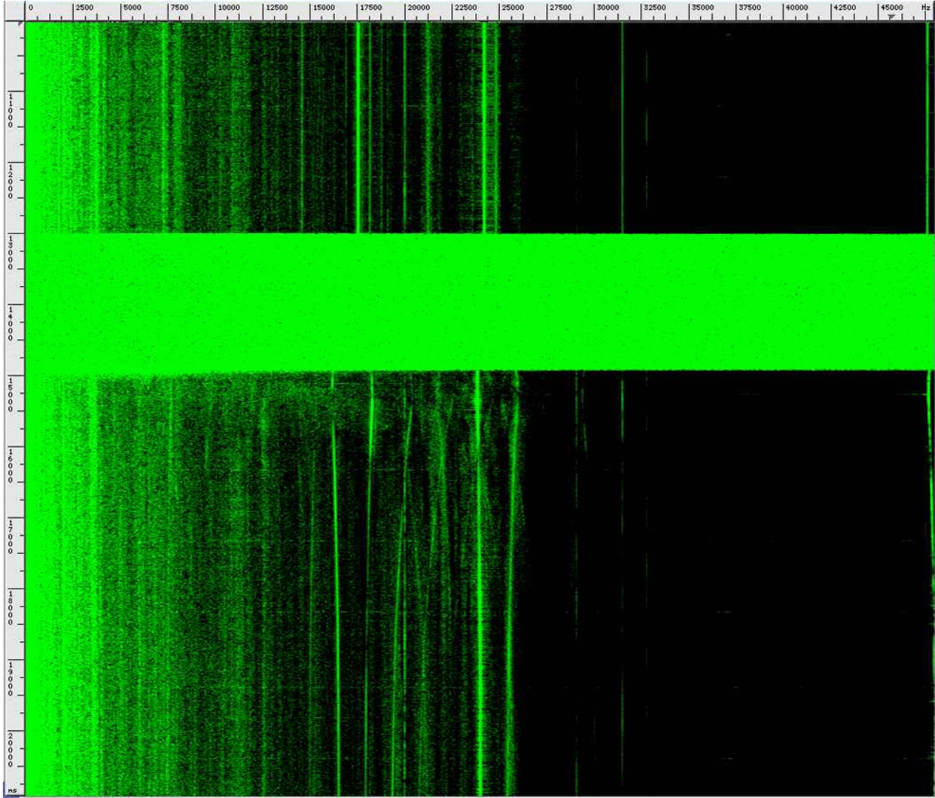
Figure 11: Acoustic measurement frequency spectrogram (2 sec, 0–45 kHz) of MUL operations while applying Quik-Freeze spray to a capacitor. After the spraying (which is loud enough to saturate the measurement), signal components shift by as much as 10Hz.
