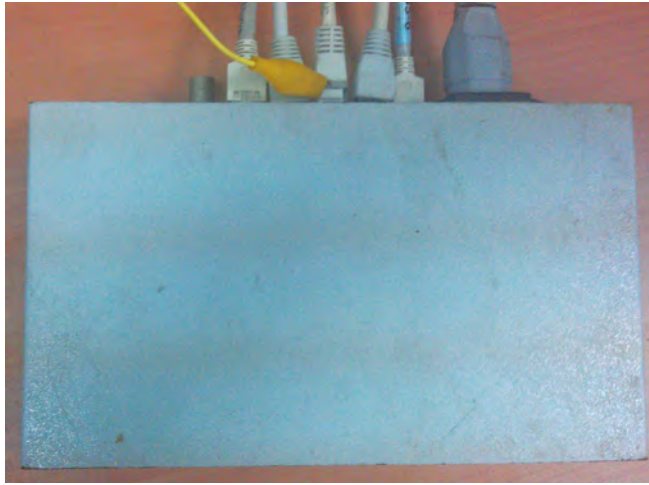
Figure 33: Chassis measurement from the far side of the Ethernet cable, while connected to an Ethernet switch. The potential is measured via the yellow clip connected to the shield of a Ethernet plug.
