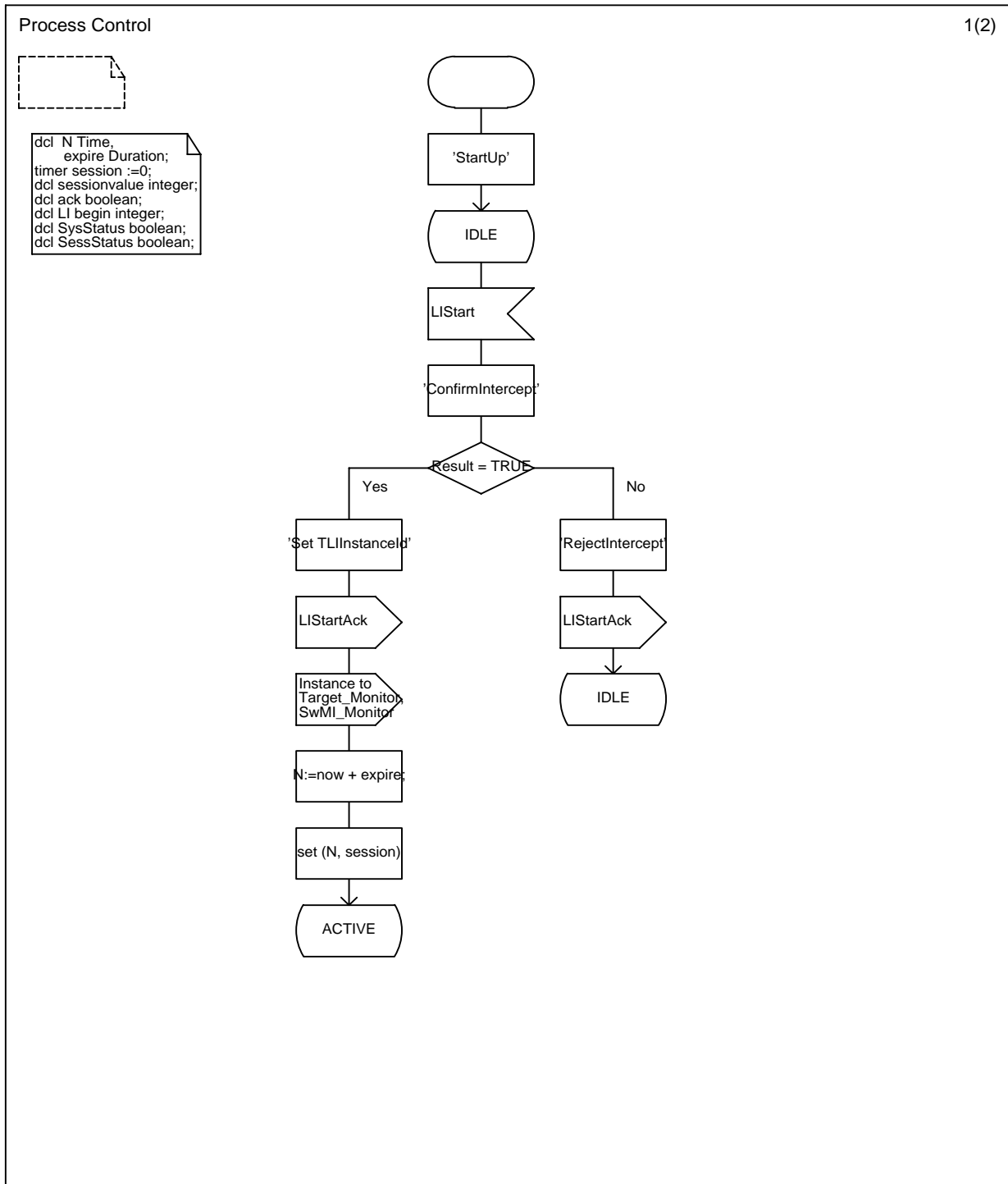
Figure B.1: Behaviour of Control process (page 1 of 2)
