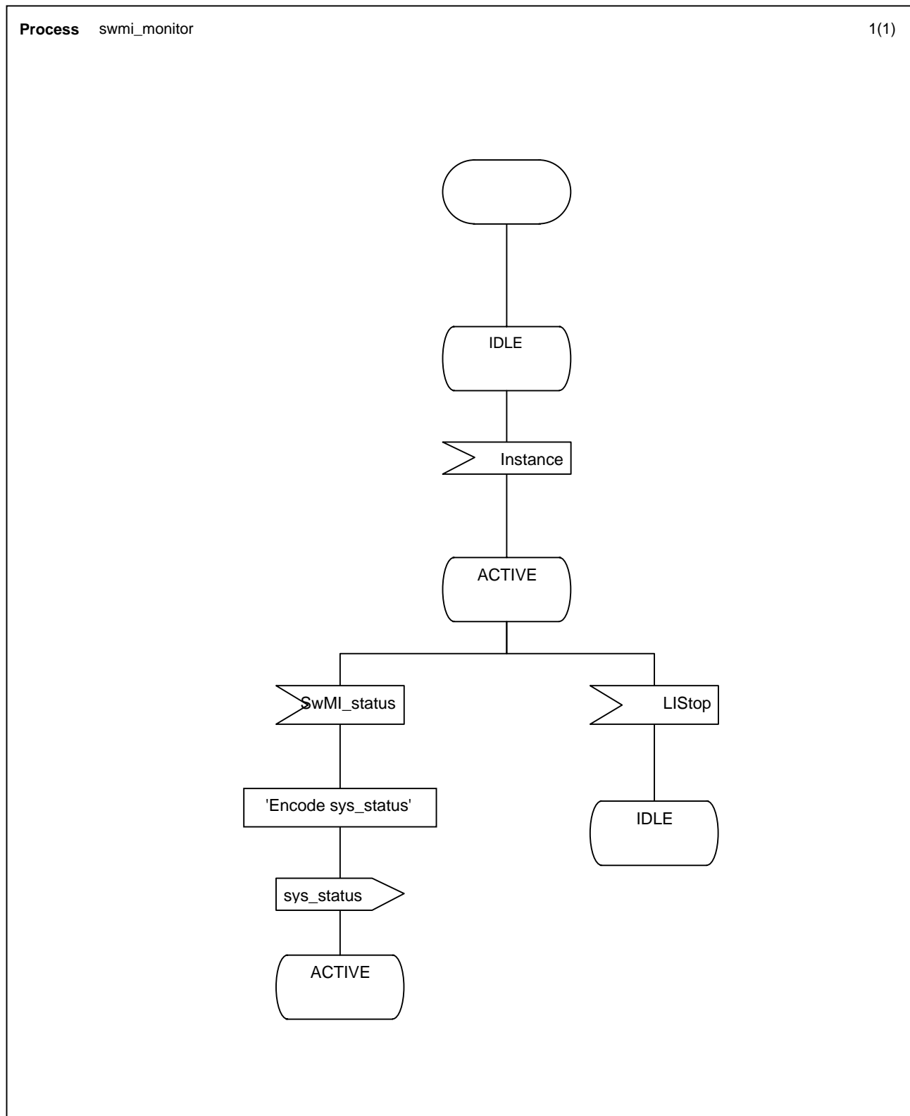
Figure B.5: Behaviour of SwMI_monitor process
