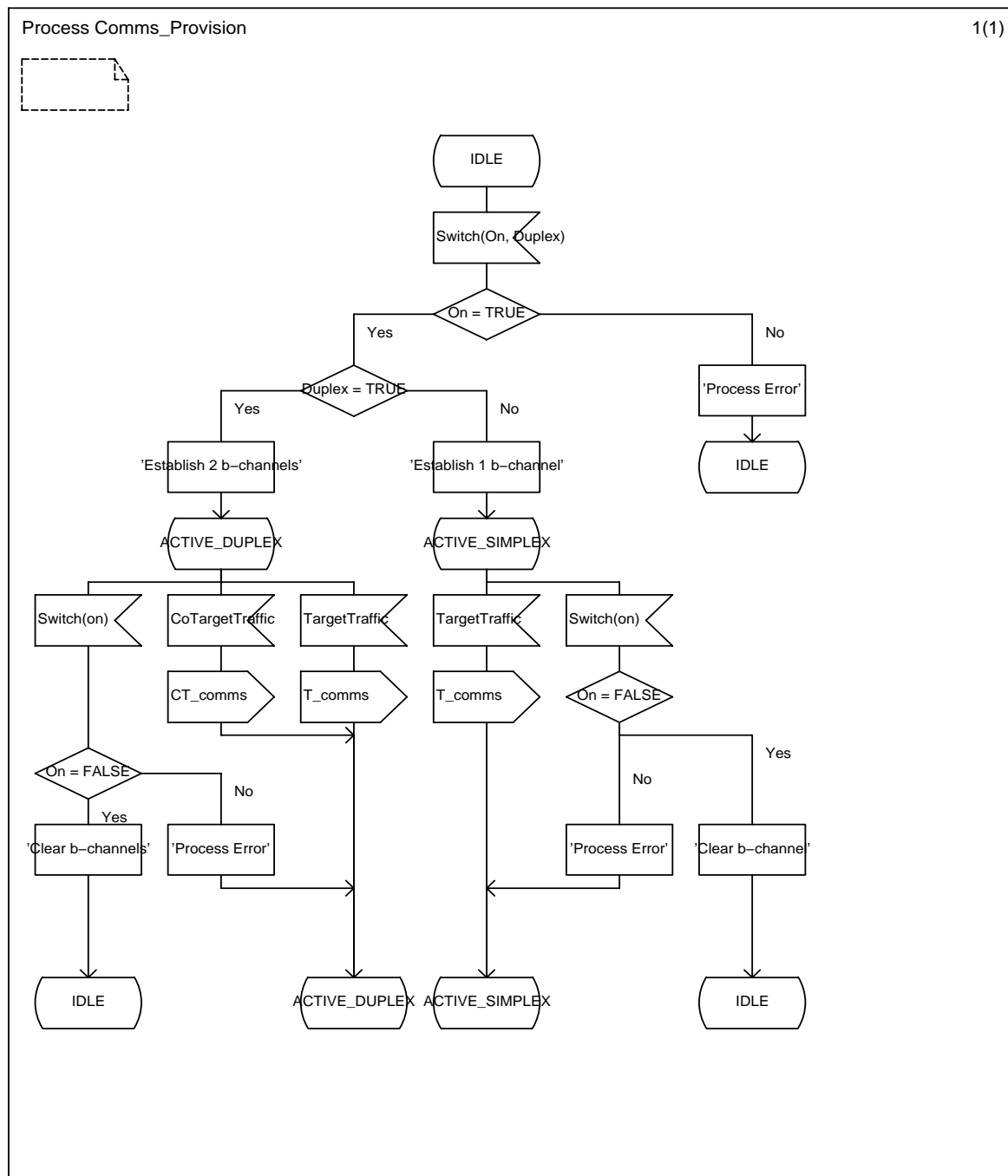
Figure B.4: Behaviour of Comms_provision process
