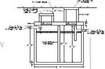
TYPICAL CYLINDRICAL 1,500 GALLON SEPTIC TANK WITH SLAB
